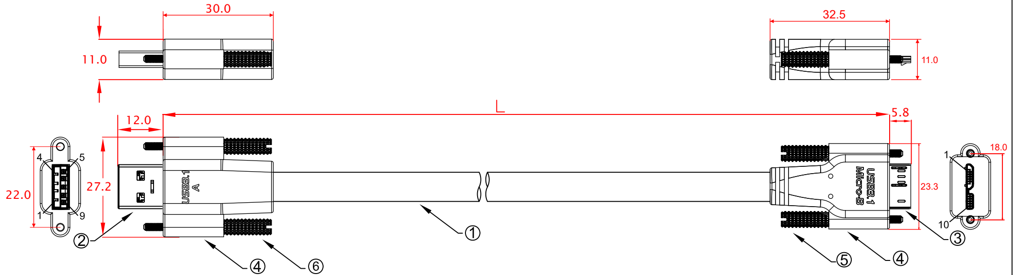
CBL-RTPD3SABMBSH-Xm with short locking screws
