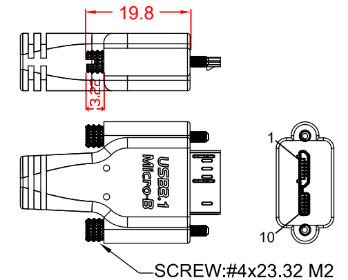
CBL-RTPD3SABMBSH-Xm with short locking screws
